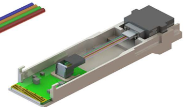
90° Bending FAU
