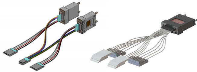
1.6T MT-FAU
